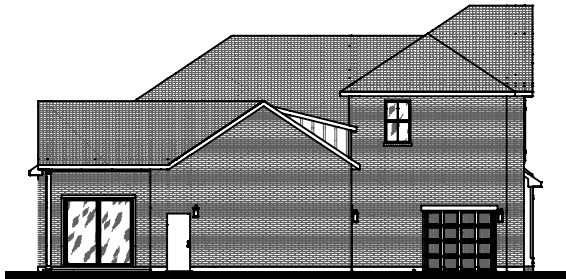
Side Elevation
