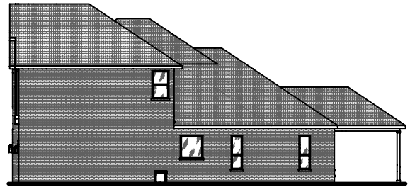
Side Elevation
