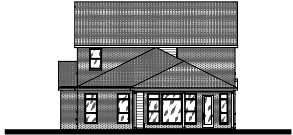
Rear Elevation
